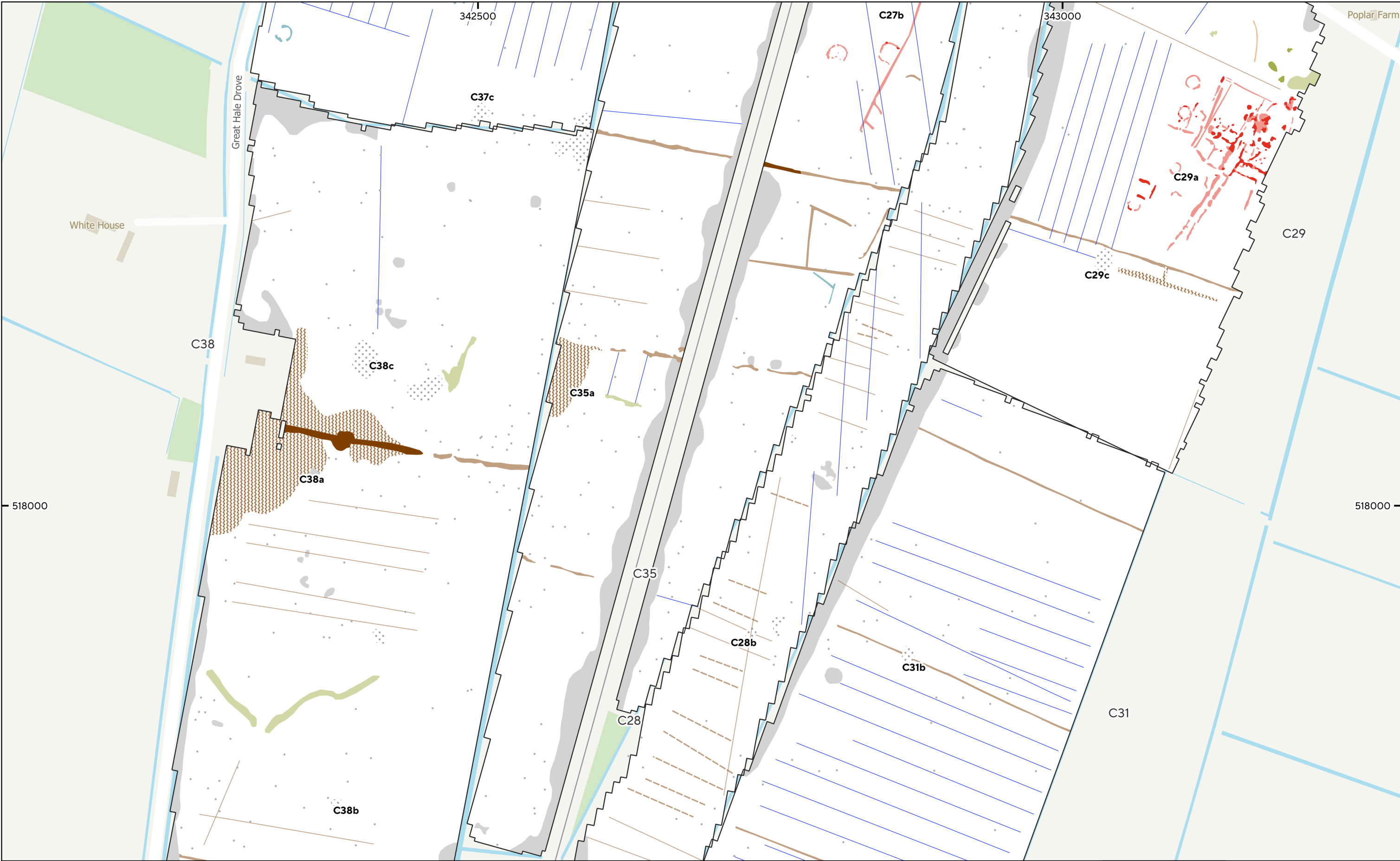
MSTF1735 - Beacon Fen Cable Route, Lincolnshire Figure 65 - Magnetic Interpretation (Cable Route Areas C27-C29, C31, C35 & C37-C38) 1:3,000 @ A3 © Magnitude Surveys 2024 Contains Ordnance Survey data © Crown Copyright and database right 2024
