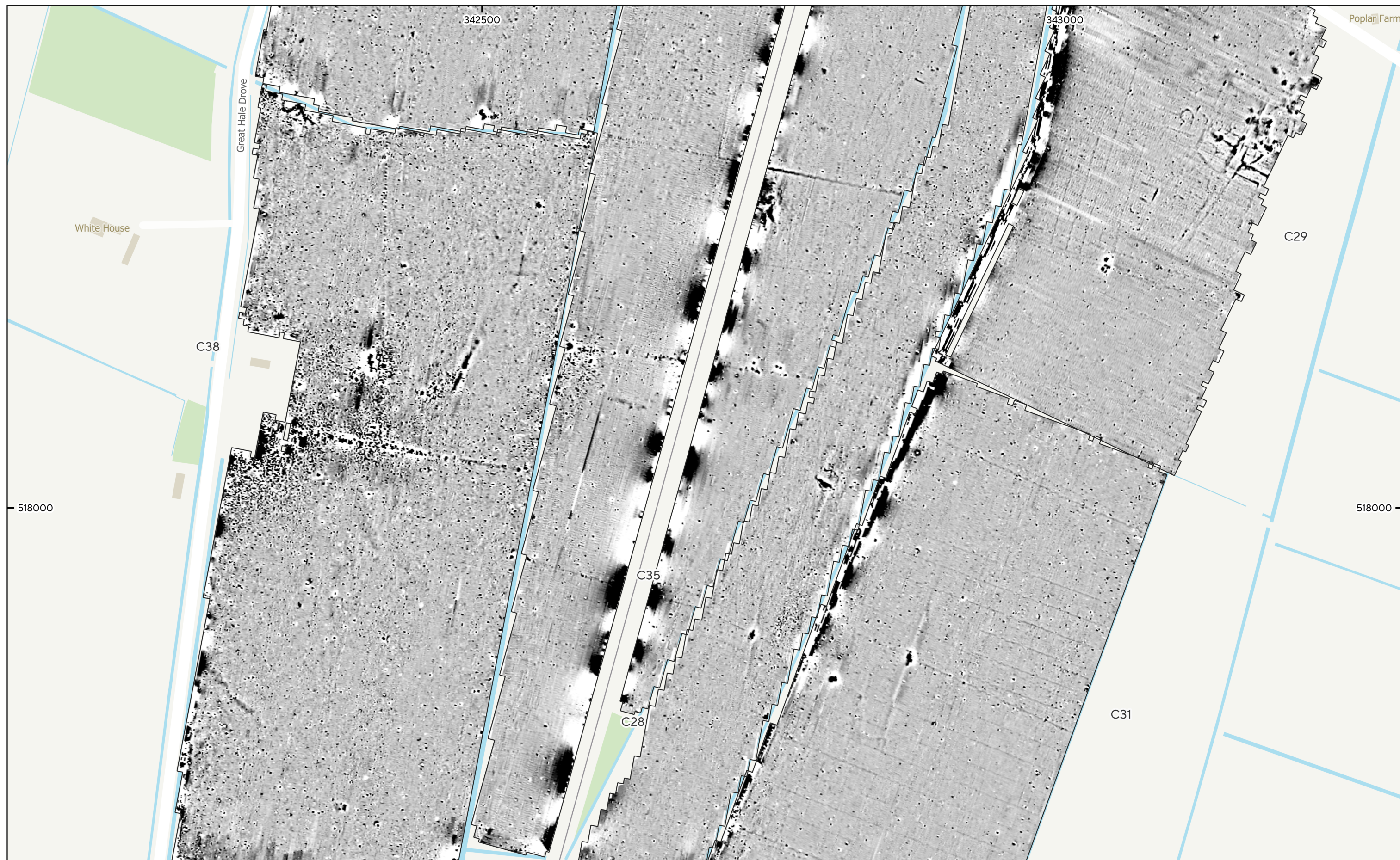
MSTF1735 - Beacon Fen Cable Route, Lincolnshire Figure 64 - Magnetic Gradient (Cable Route Areas C27-C29, C31, C35 & C37-C38) 1:3,000 @ A3 © Magnitude Surveys 2024 Contains Ordnance Survey data © Crown Copyright and database right 2024
